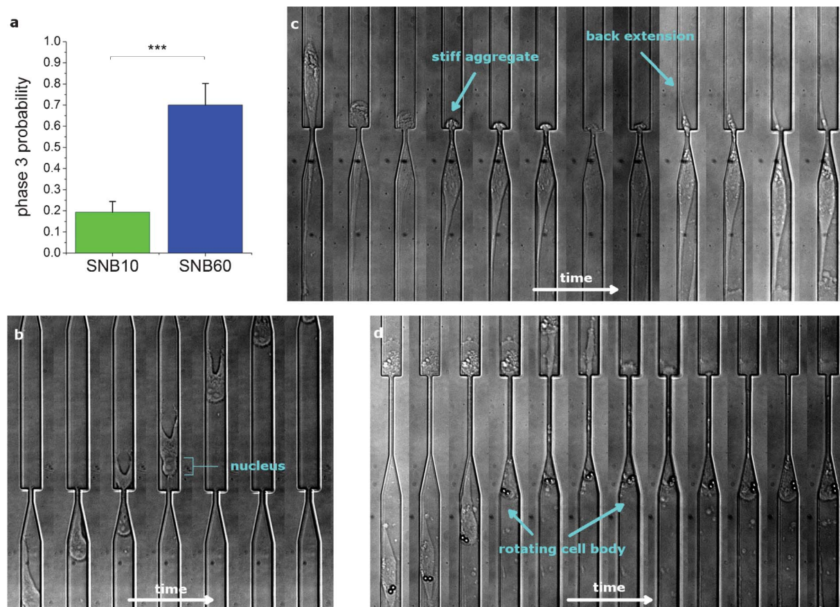
Fig. 3 Functional strategies during mechanical invasion. a) The probability of phase 3 existing for the two different subnucleus barriers SNB10 and SNB60. SNB60 induces a higher probability of phase 3 existing (70%, n = 20 ) than SNB10 (19.4%, n = 62 ). Error bars represent standard error of the mean (s.e.m.) from Bernoulli statistics and *** indicates p < 0.001 (Chi-squared test). b) A timelapse image stack (17 min/frame) showing a cell invading across SNB10 with no phase 3 observed. The contractile force of the cell is enough to deform the cell nucleus across the barrier in a monotonic forward motion. c) As this cell invades from top to bottom across SNB60, a stiff aggregate at the rear of the cell is stuck at the barrier interface. A back extension is protruded, which tensionally reduces the width of the aggregate and facilitates intracellular trans -barrier transport. 34 min elapsed between subsequent frames. d) As this cell is invading from the LC into SNB60, cell body rotations, with visualization facilitated by endocytosed particles, can be seen in the timelapse image stack during the invasion process. These rotational dynamics may help position the cell more favorably and/or sample more energetically favorable conformations as the cell is invading across the subnucleus barrier. 34 min elapsed between subsequent frames. The width of the larger channel is 15 \mu\text{m} .
