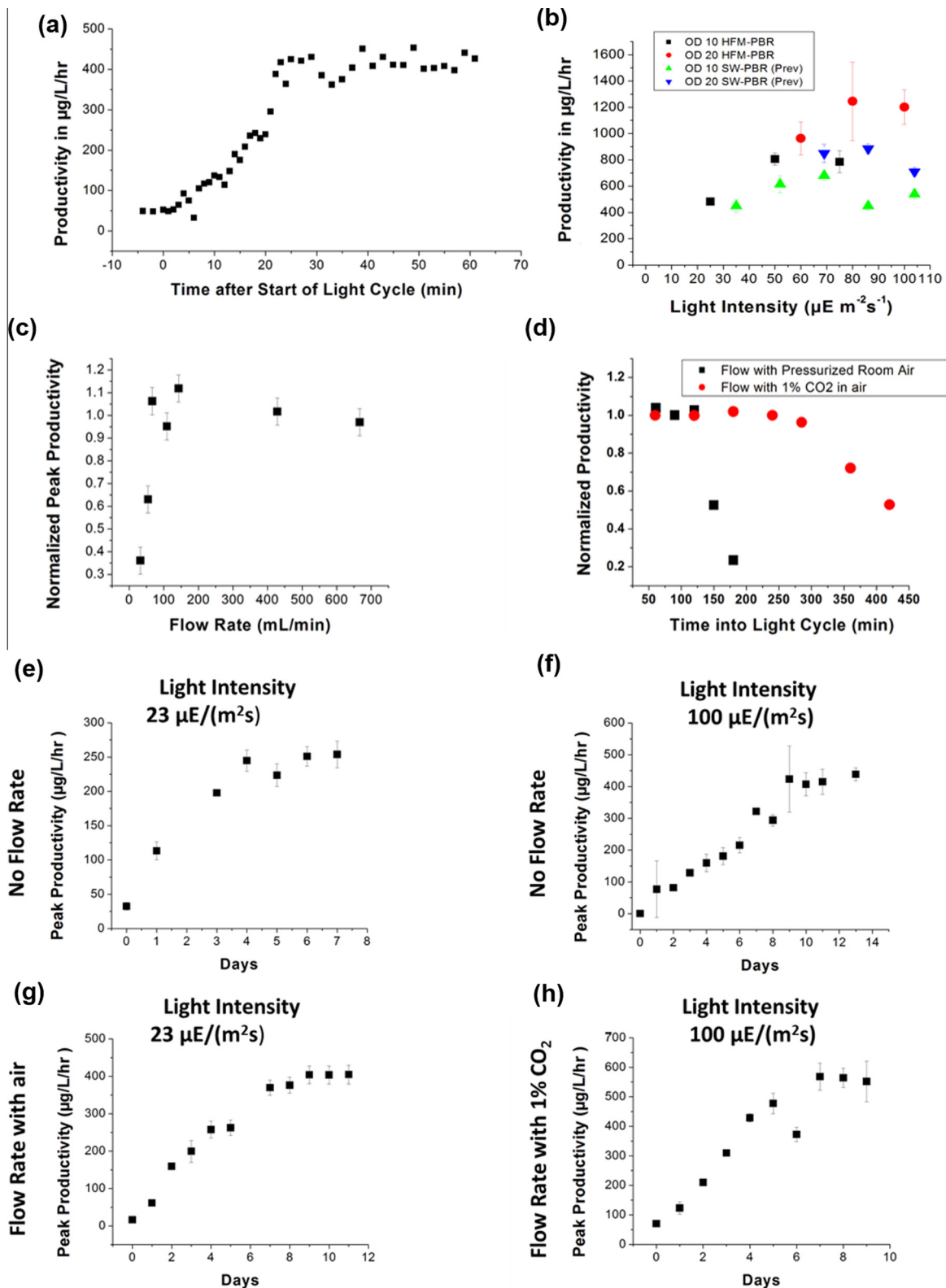
Fig. 1. (a) Transient behavior at beginning of light cycle; (b) peak productivity with carbonated gas stream at different intensities loaded with high \text{OD}_{730} cultures; (c) normalized productivity to flow rate; (d) normalized productivity over course of light cycle for different gas streams. Growth experiments performed at (e) low light intensity and passive aeration; (f) high light intensity and passive aeration; (g) low light intensity and active aeration with air; (h) high light intensity with active aeration with 1% \text{CO}_2 .
